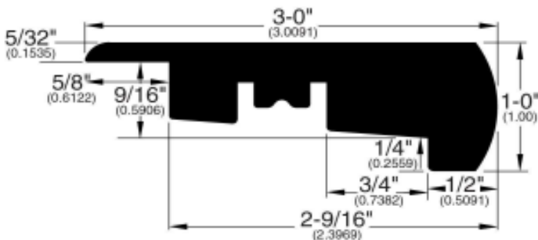
Overlap Stair Nose (292)
