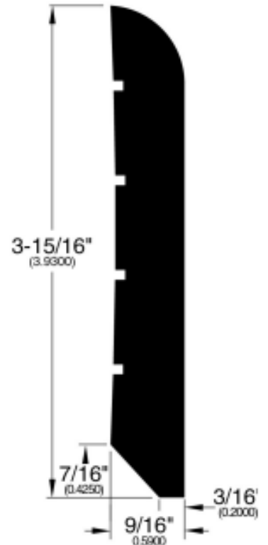
Wall Base (294)
