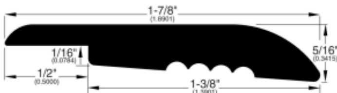
Overlap Reducer (297)
