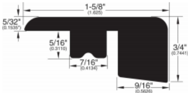
Square Nose (338)
