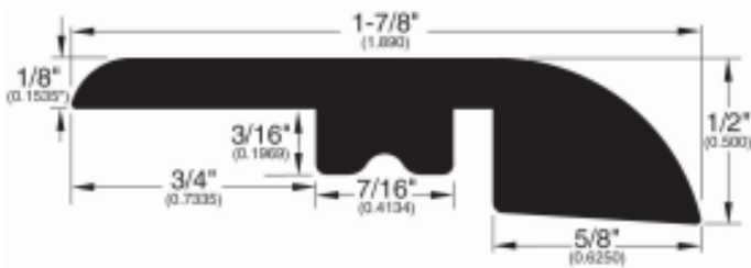
Overlap Reducer (290)
