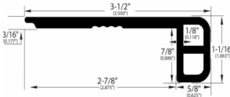
Stair Nose (340)
