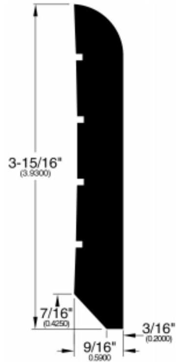
Wall Base (294)
