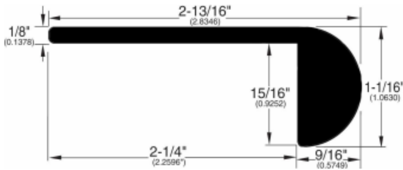
Stair Nose (298)
