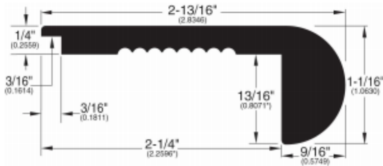
Stair Nose (288)
