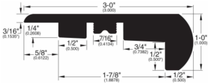
Overlap Stair Nose (283)
