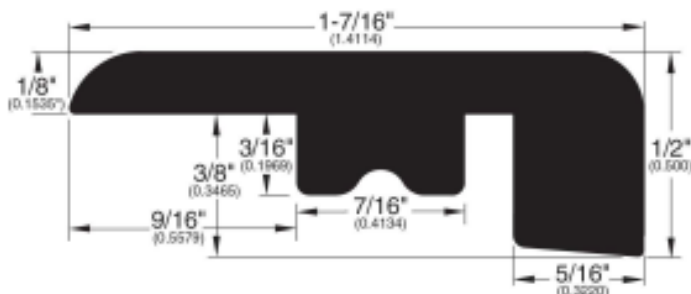
Square Nose (291)
