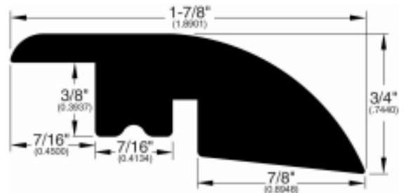
Overlap Reducer (293)
