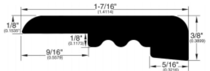
Square Nose (300)
