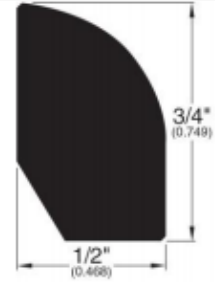
Base Shoe (024)
