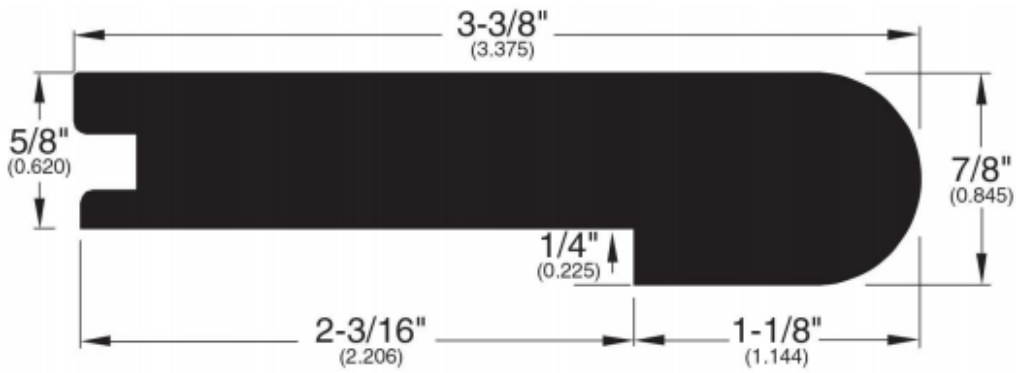
Stair Nose (069)
