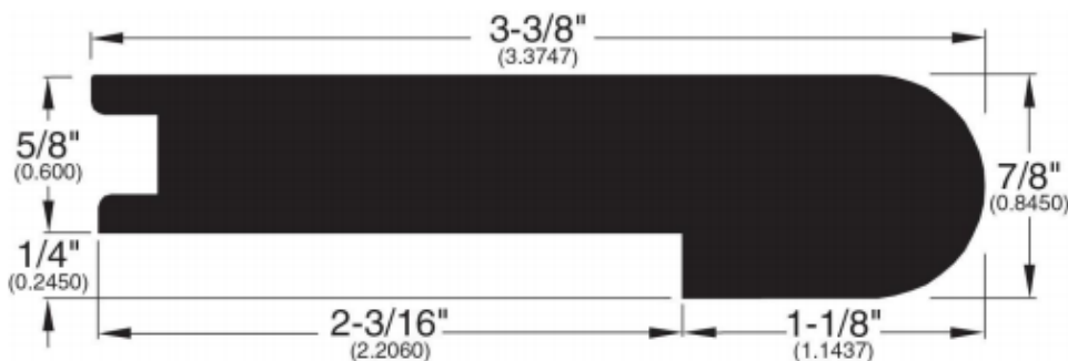
Stair Nose (038)
