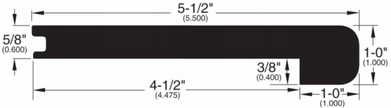
Stair Nose (222)
