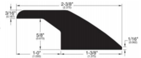
Reducer Overlap (025)
