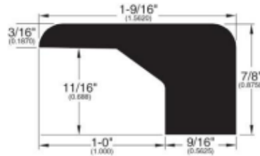
Square Nose (027)
