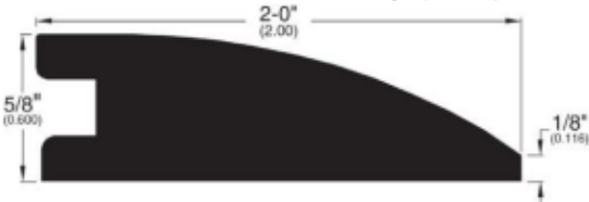
Reducer (037)
