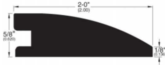
Reducer (068)
