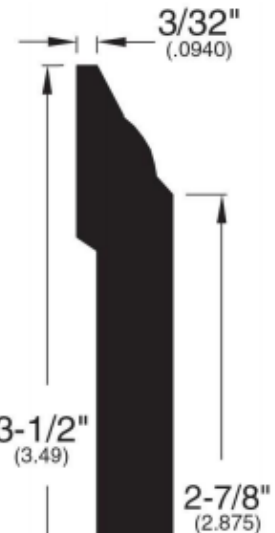
Reducer Overlap (025)
