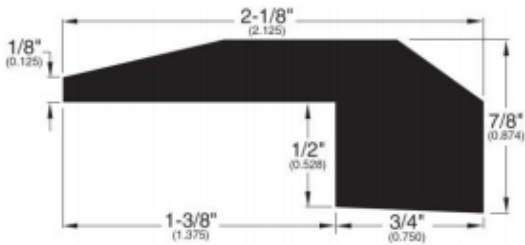
Threshold (011)
